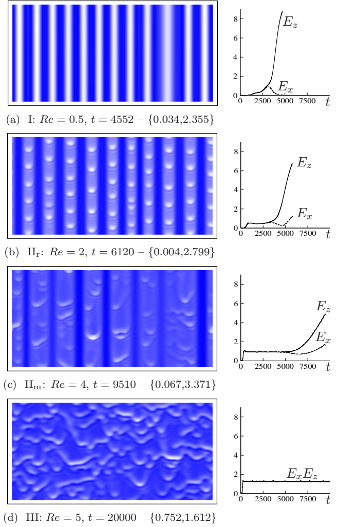
Fig. 2: Typical wave pattern for each regime (or phase). See legend of fig. 1. The times for (a-c) are near rupture. Plots show streamwise ( E_x ) and transverse ( E_z ) energies of deformations.
