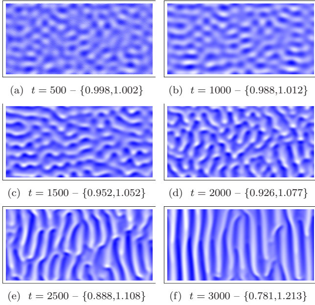
Fig. 1: Water film free surface at different times for Re = 0.5 . Bright (dark) zones correspond to elevations (depressions) of the film whose extrema are given in brackets.
