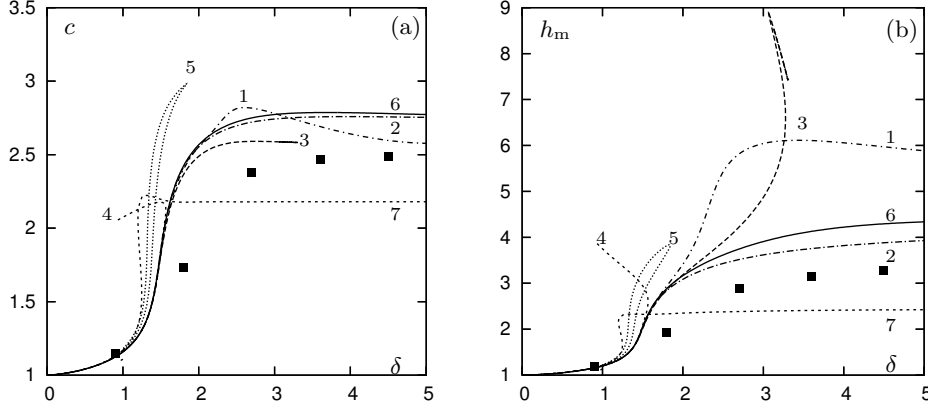
FIGURE 1. Speed c (a) and amplitude h_m (b) of the principal homoclinic orbits as functions of the reduced Reynolds number \delta . The wall is vertical and streamwise viscous dissipation is omitted ( \zeta = \eta = 0 ). 1: complete second-order model (3.1,C 1); 2: simplified model (3.1,4.1); 3: (3.1, 4.4) with \mathcal{K} given by (4.5); 4: with \mathcal{K} given by (4.7); 5: with \mathcal{K} given by (4.8); 6: regularised model (3.1, 4.15); 7: PMB model (3.1, 3.6); filled squares: solutions to the first-order boundary-layer equations after Chang et al. (1996).
